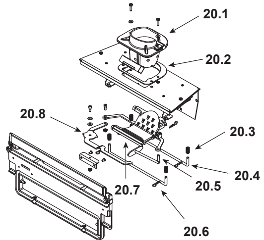
#20 Firepot Riser Assembly
