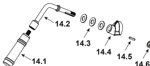
#14 Handle Assembly
