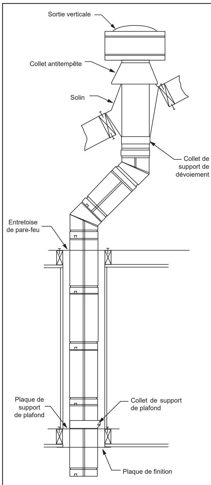
Figure 3.16 – Configuration typique de ventilation verticale
