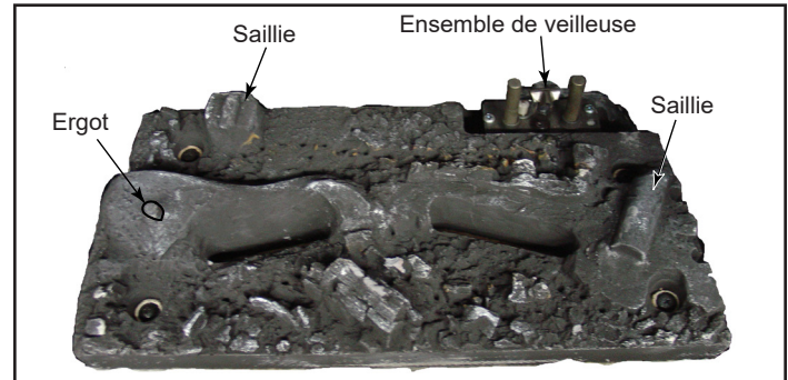
Figure 3.26 – Bûche arrière
