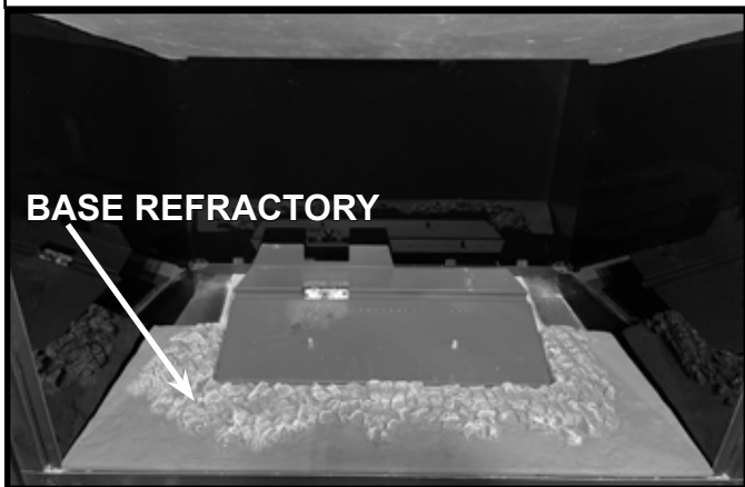
Figure 15 Type 1 Base Refractory Installed (One Piece Model)
