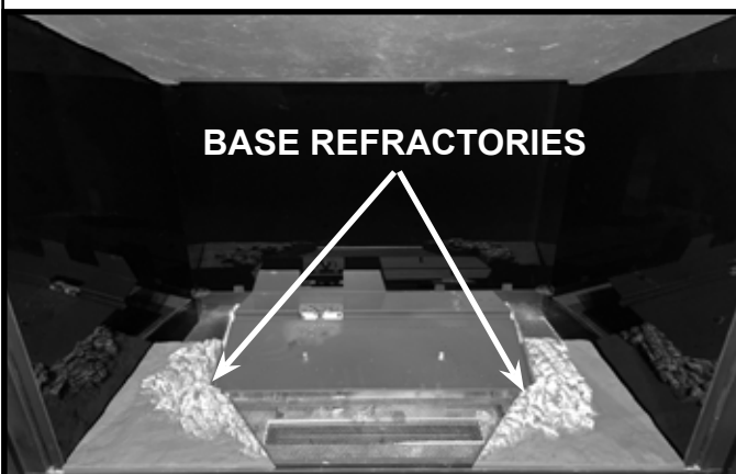
Figure 16 Type 2 Base Refractory Installed (Two Piece Model)
