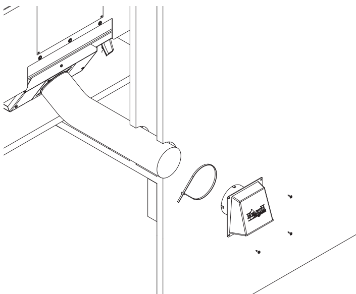
Figure 16.1 - Installation arrière
