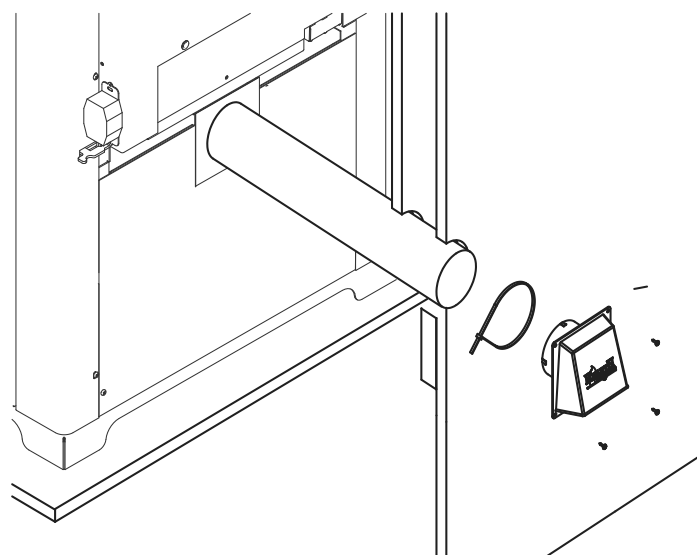
Figure 16.1 - Installation arrière
