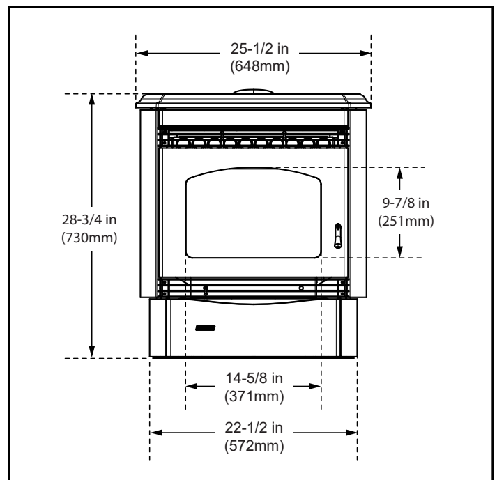
Figure 8.4 - Front View
