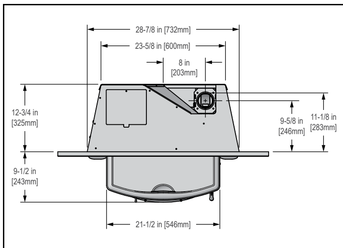
Figure 8.1 - Top View
