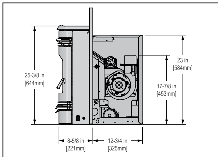
Figure 8.3 - Side View
