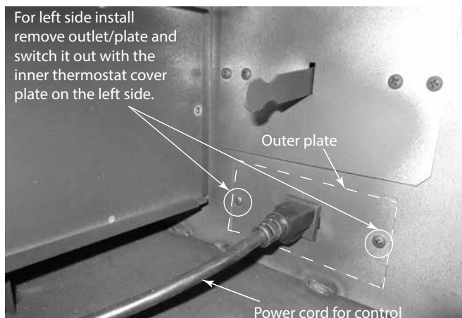
Figure 4.4 Junction Box Shown on Right Side
