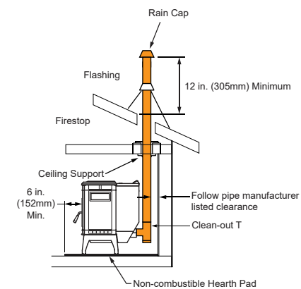
Vertical - Interior, Preferred Installation
