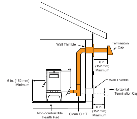
Exterior - Optional Installations
