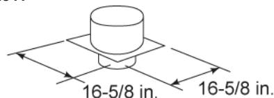
MH842 Roof Flashing & Thimble
