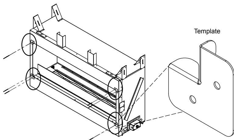
Figure 1. Drill corner holes using provided template
