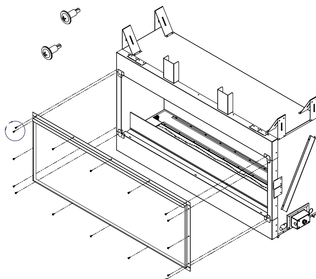
Figure 2. Install The top bottom and side trims
