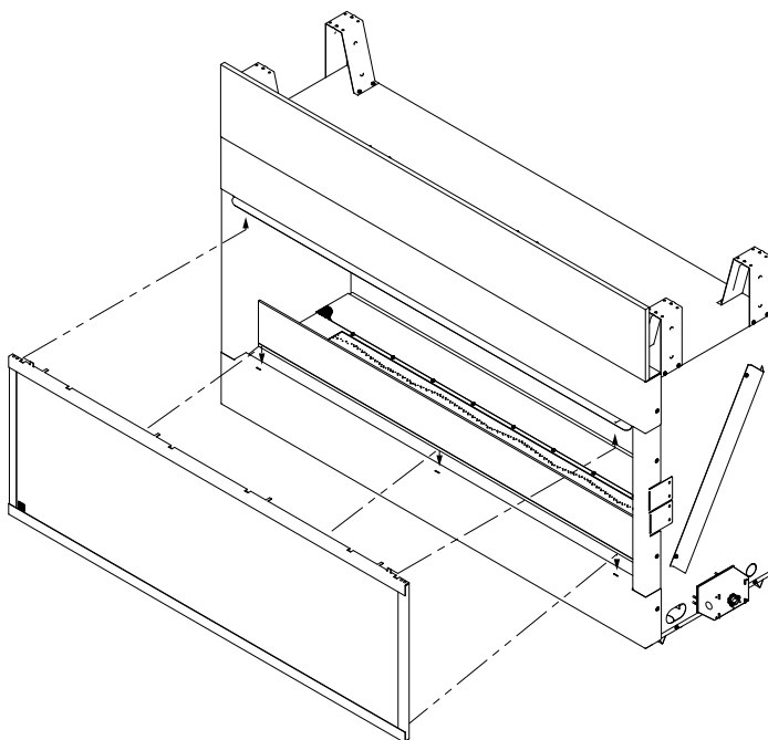
Figure 1. Installing the Screen
