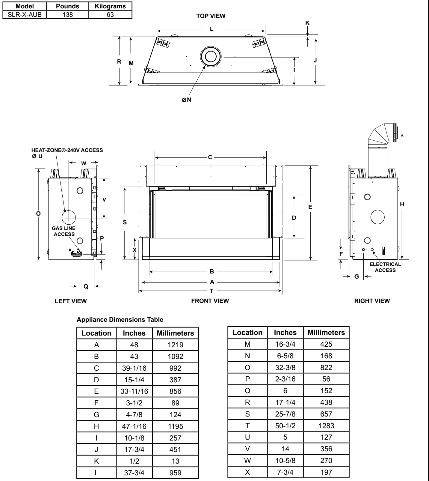
Figure 3.1 Appliance Dimensions
