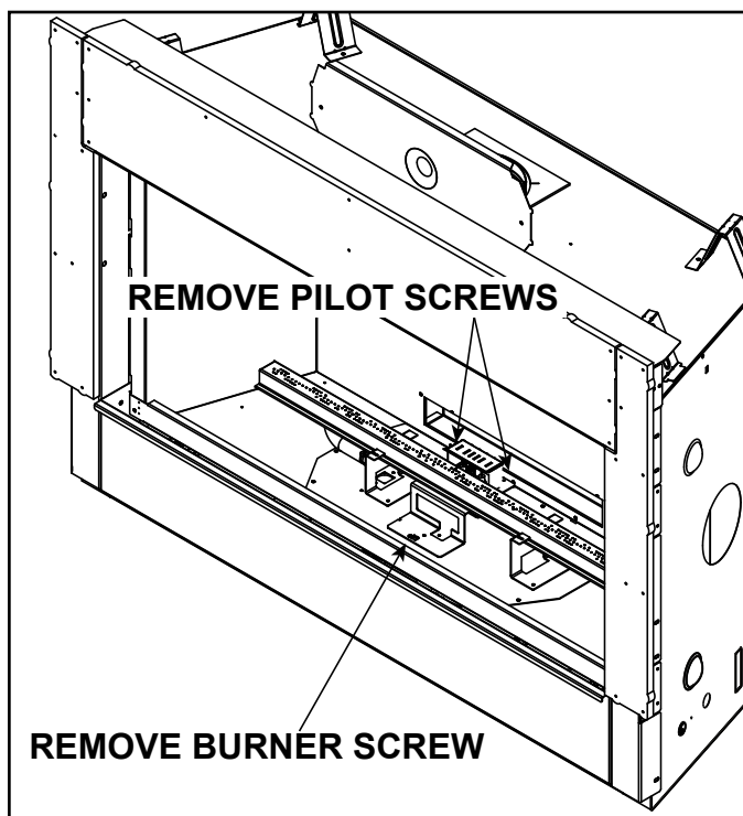
Figure 9.2 Burner Removal
