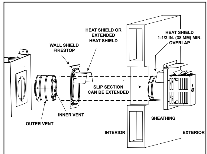
Figure 7.13 Venting Through the Wall
