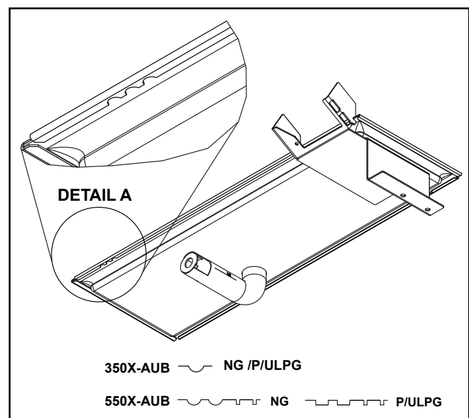
Figure 9.2 Burner Identification
