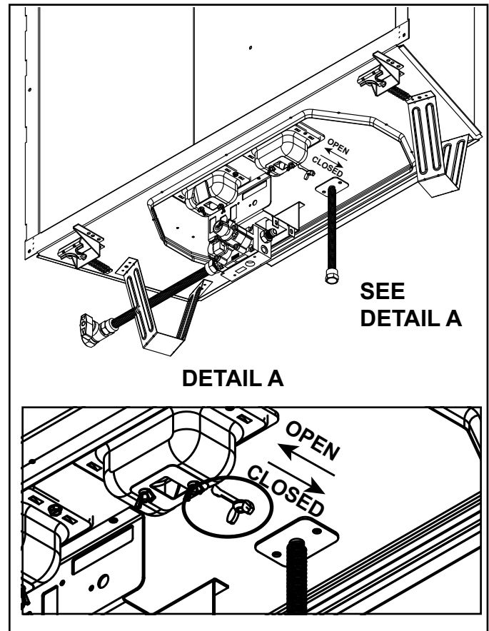
Figure 9.1 Air Shutter Adjustment
