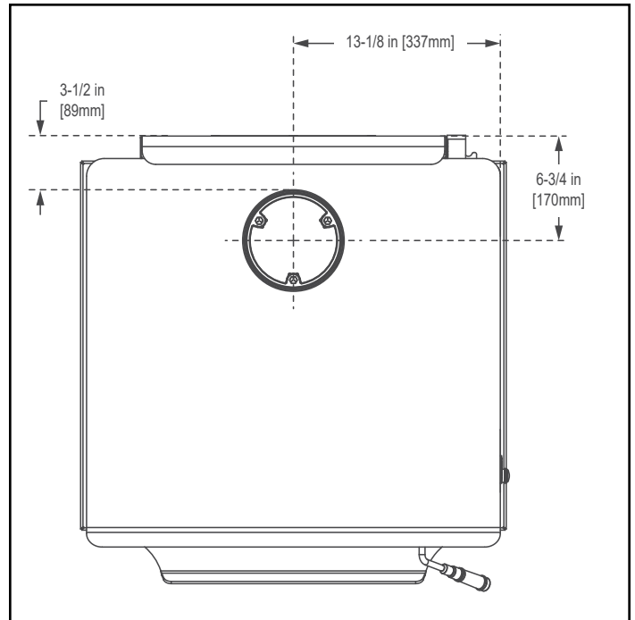
Figure 8.2 - Top View
