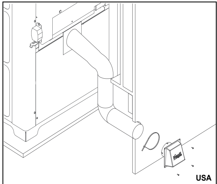
Figure 16.2 - Floor Installation
