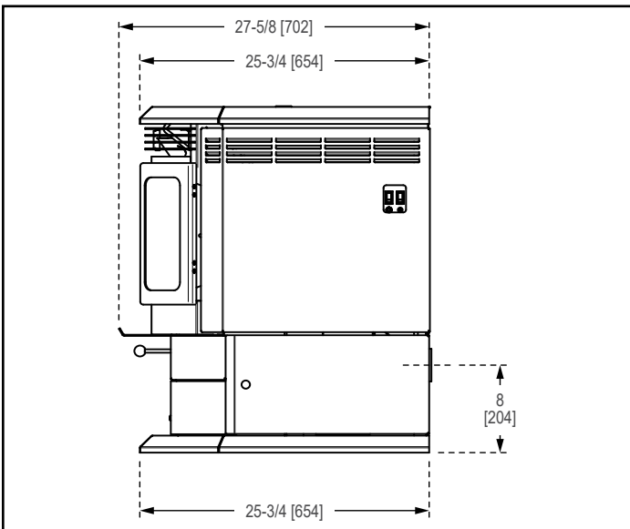
Figure 8.2 - Side View
