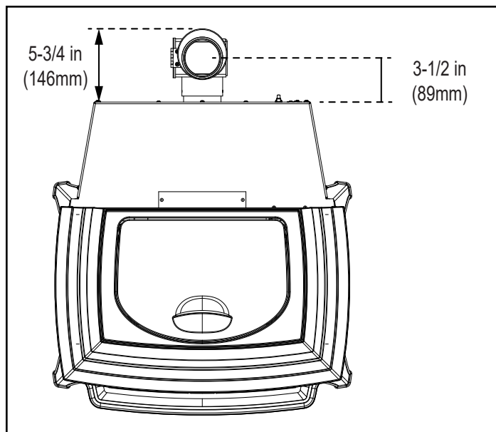
Figure 8.3 - Top View with TPVNT-6 and 811-0720
