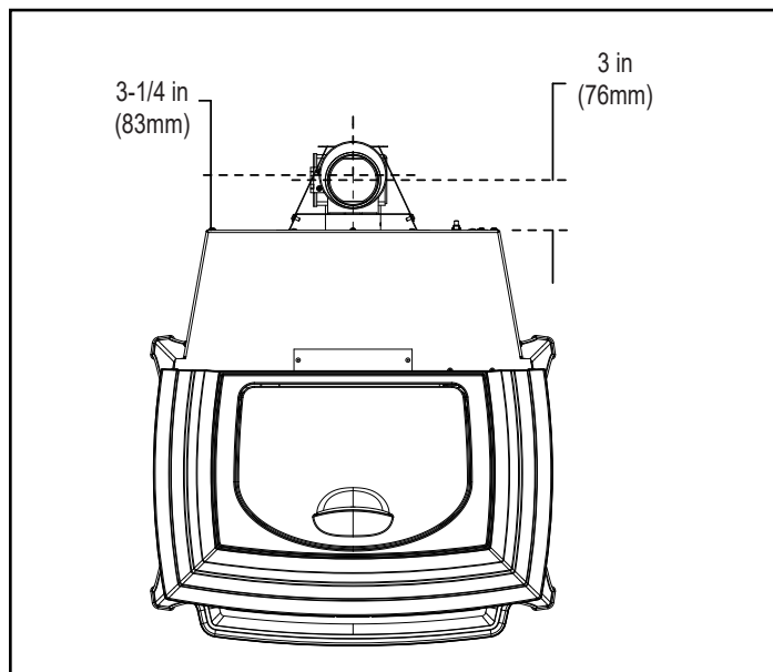
Figure 8.4 - Top view with TPVNT-2 and 811-0720
