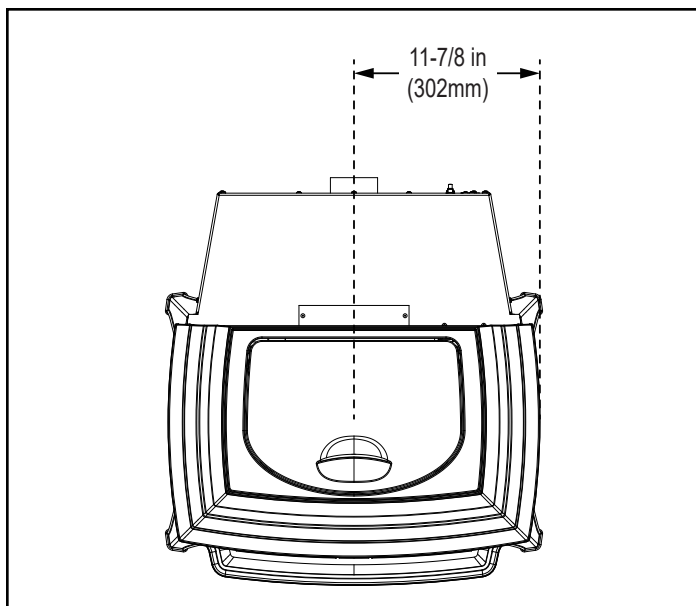
Figure 8.1 - Top View
