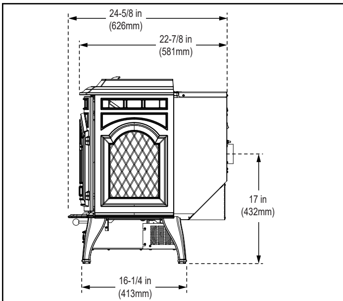
Figure 9.2 - Side View
