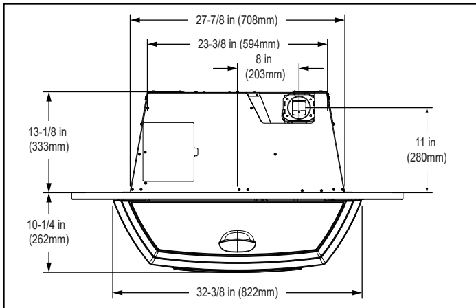
Figure 8.1 - Top View with Small Surround Panel Set
