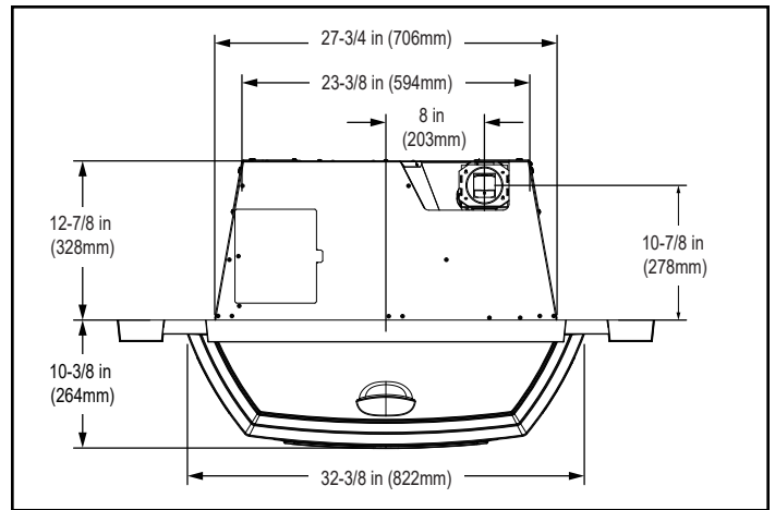
Figure 8.4 - Top View with Cast Panel Set
