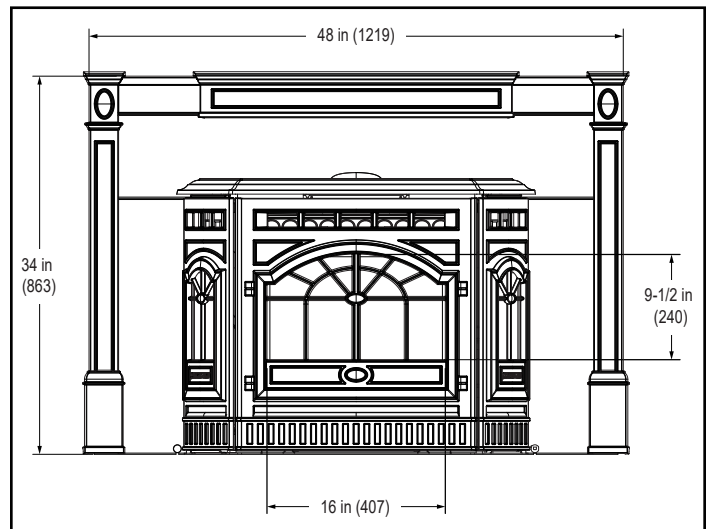
Figure 8.6 - Front View with Large Surround and Cast Panel Set
