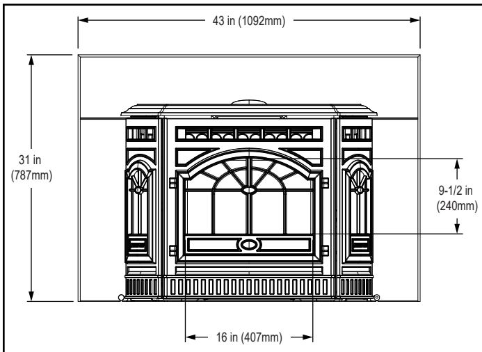
Figure 8.2 - Front View with Small Surround Panel Set
