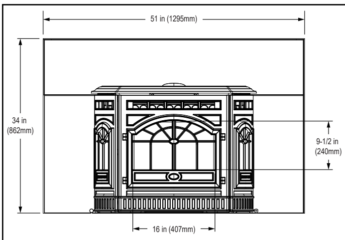
Figure 8.3 - Front View with Large Surround Panel Set
