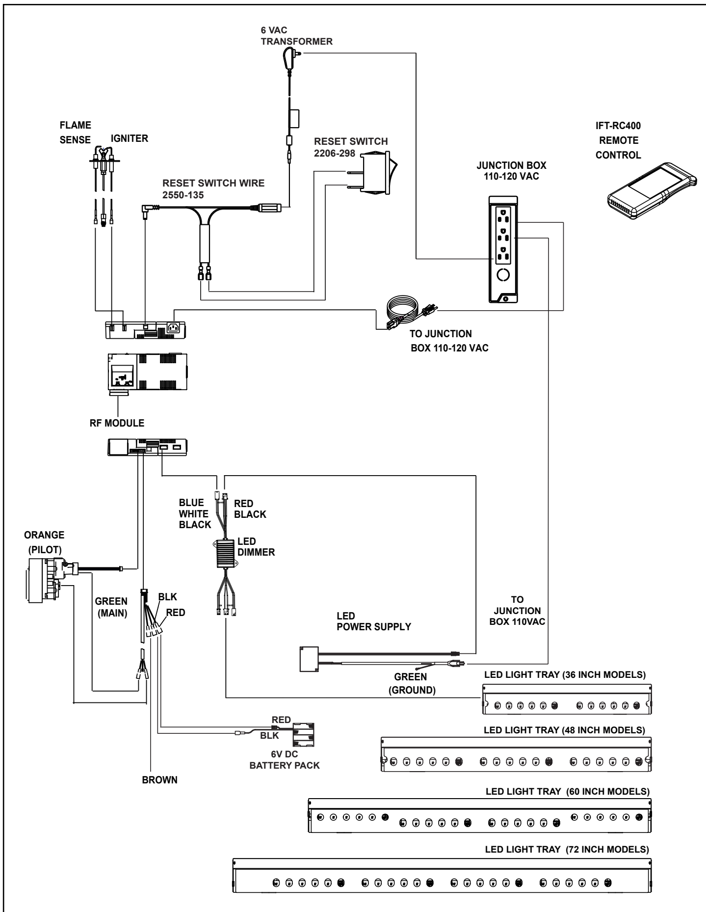
Figure 5 LED Wiring Diagram
