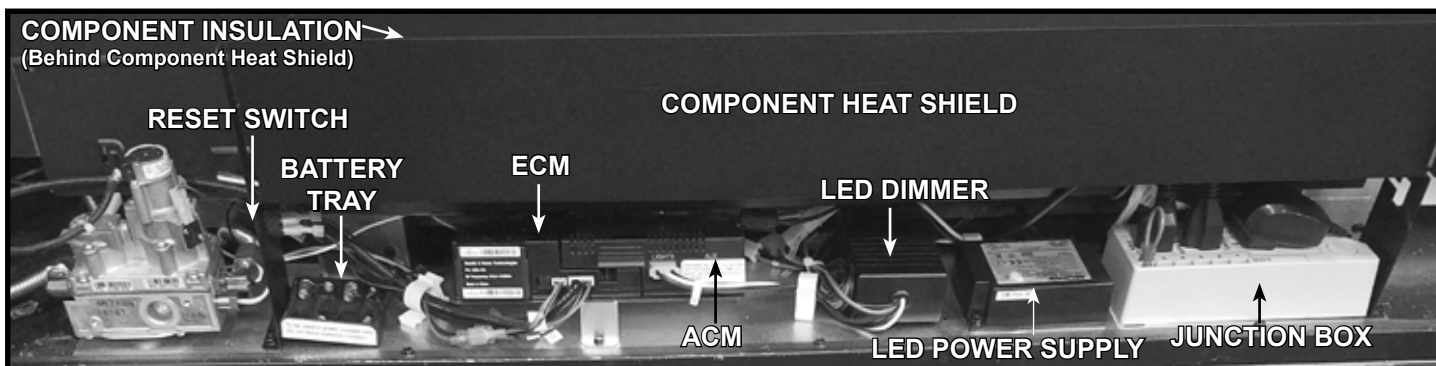
Figure 3 Valve Cavity (Lower Access Panel Removed)
