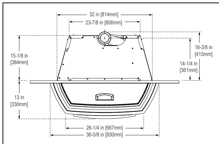
Figure 8.4 - Top View with Basic Surround Panel Set
