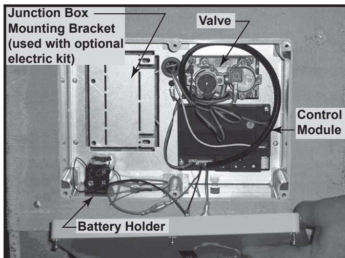
Figure 5.3 Control Box
