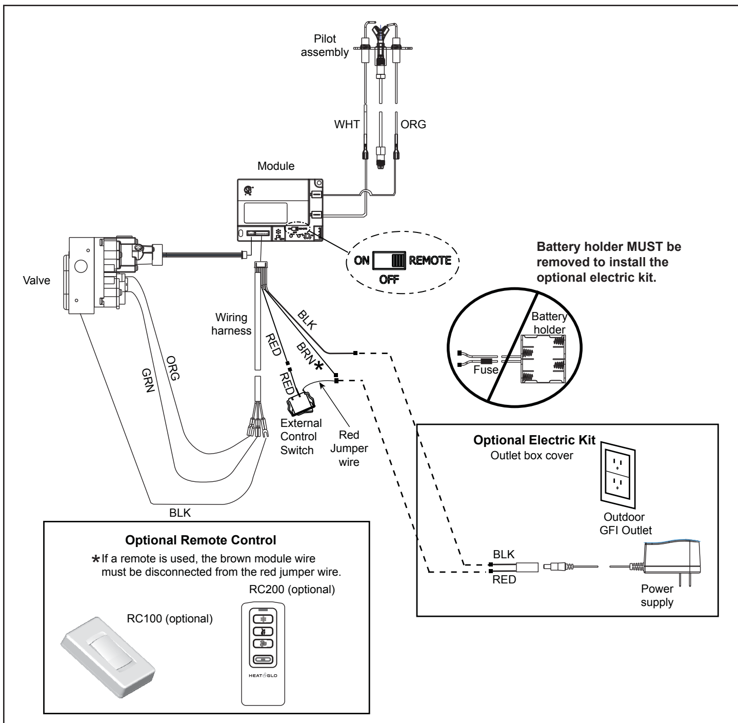
Figure 6.12 Intermittent Pilot Ignition (IPI) Wiring Diagram with Optional Electric Kit and Optional Remote Control
