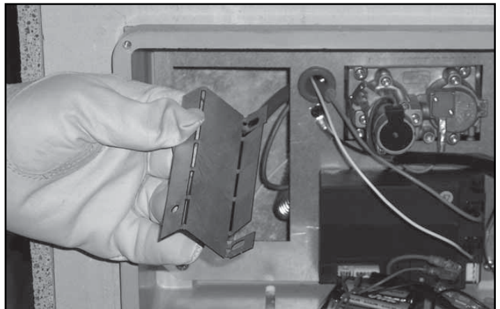
Figure 6.6 Hand-bend Bracket
