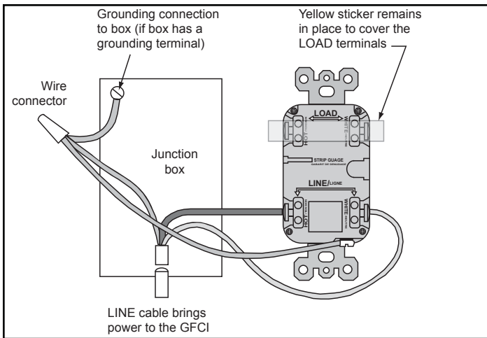
Figure 6.9 Wire the GFI Receptacle
