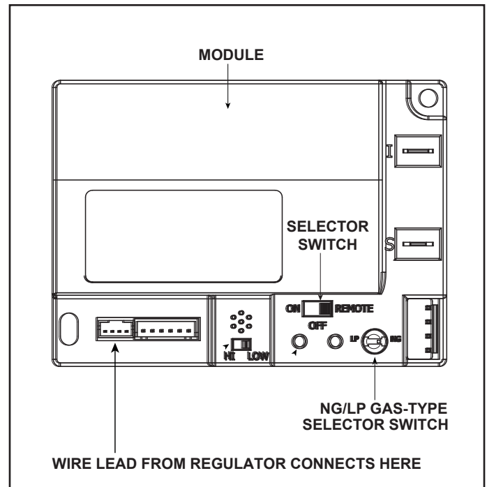
Figure 6.2 Control Module
