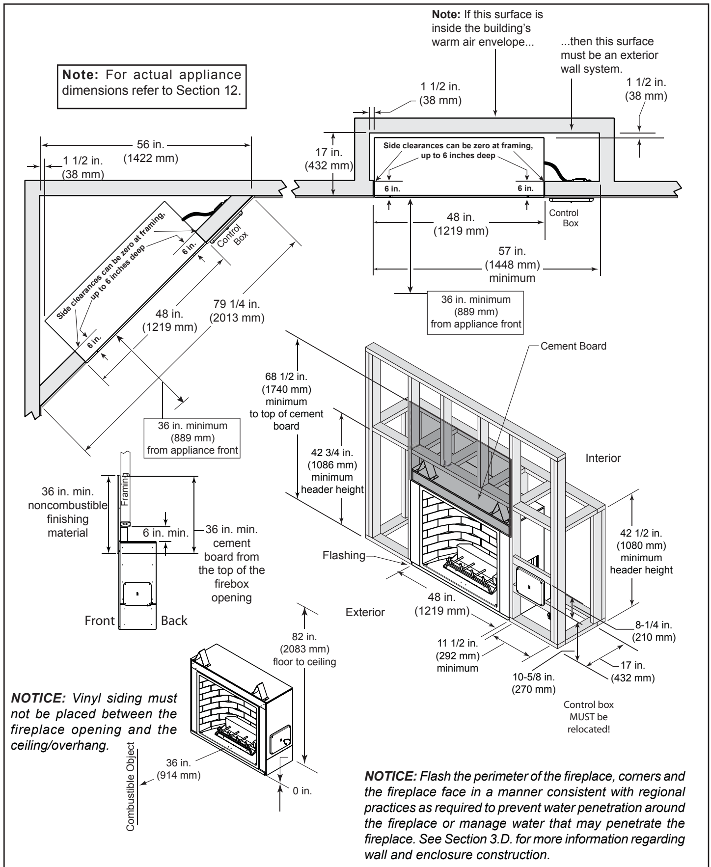
Figure 3.1 Appliance Locations and Framing Dimensions - CARODG36I, CARODG36IL
