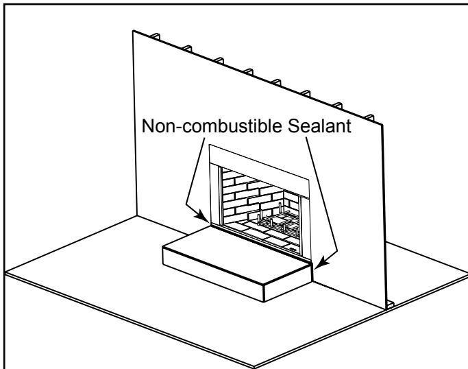
Figure 7.11 Place Non-combustible Sealant
