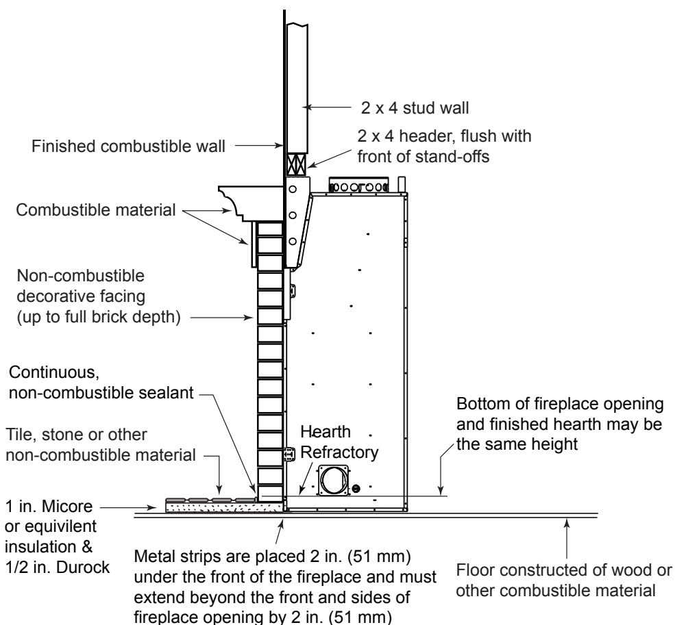
Figure 12.10 Decorative Facing
