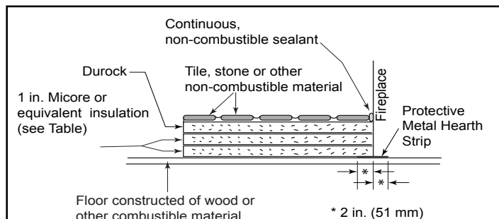
Figure 12.2 Hearth Extension Construction
