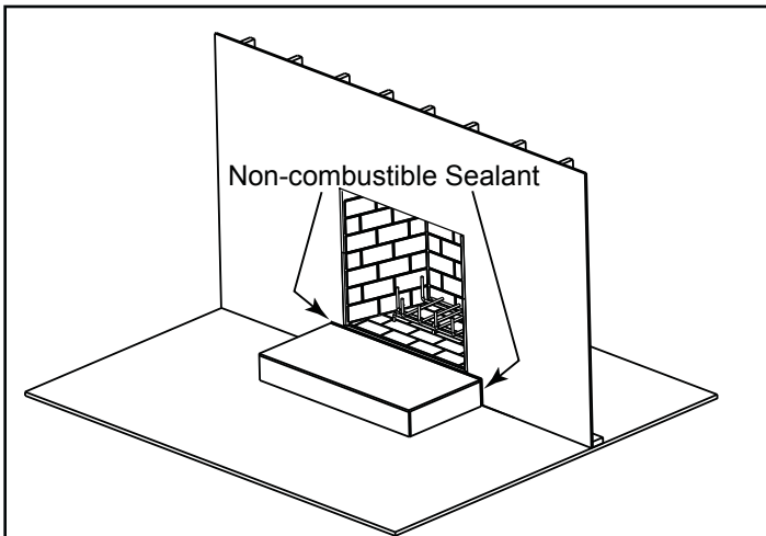
Figure 12.6 Place Non-combustible Sealant
