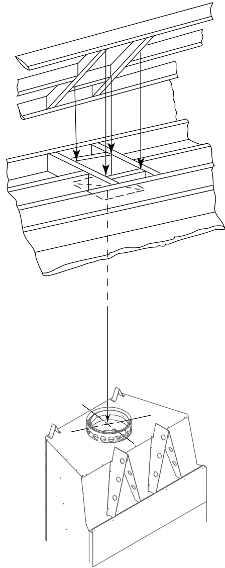
Figure 8.9 Ceiling/Attic Construction
