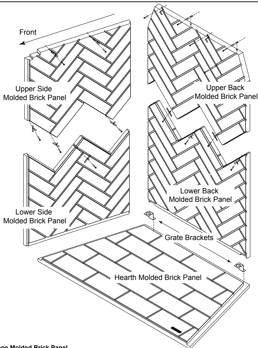
Figure 11.2 Herringbone Molded Brick Panel
