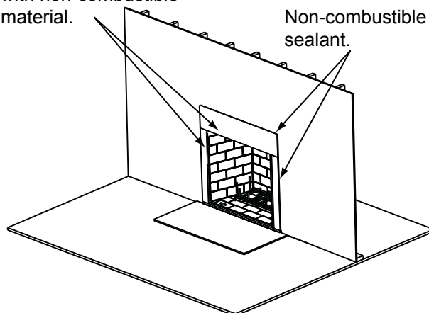
Figure 12.9 Non-combustible Facing
