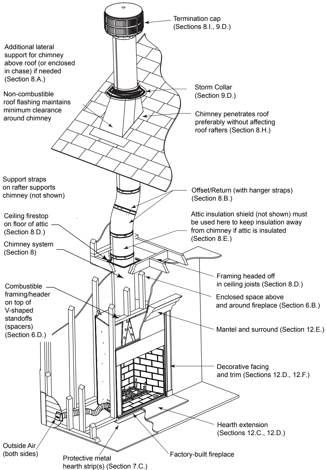
Figure 5.1 Typical Fireplace System
