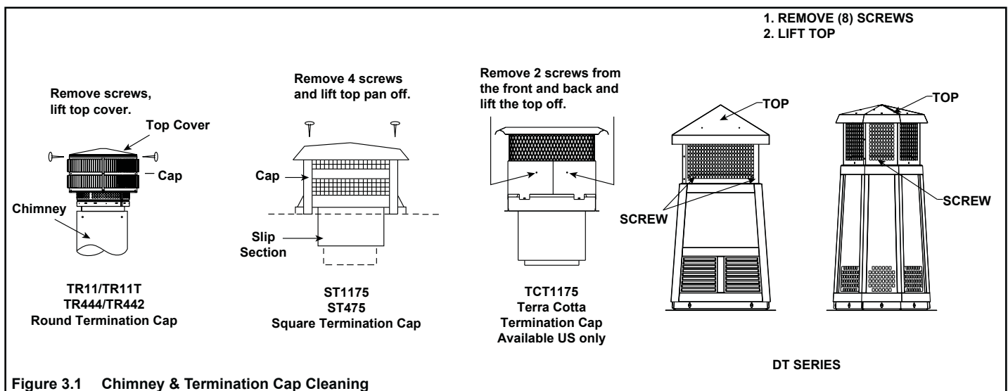
Figure 3.1 Chimney & Termination Cap Cleaning
