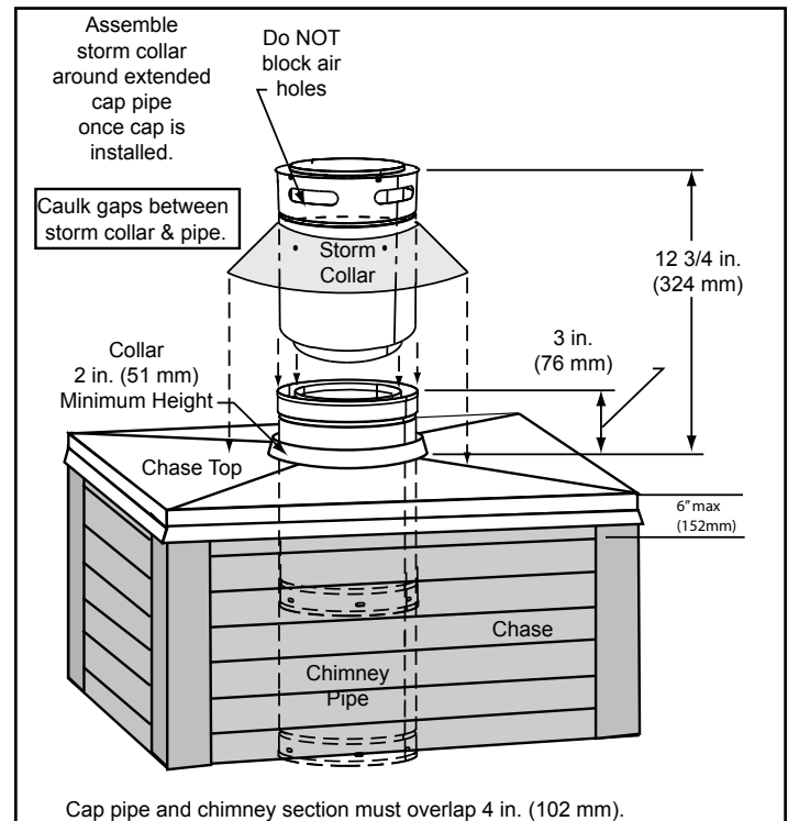
Figure 3 Installing CT-14A Cap Adapter
