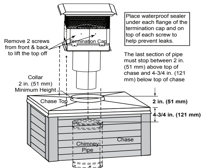
Figure 5.14 Installing a TCT375 Terra Cotta Cap
