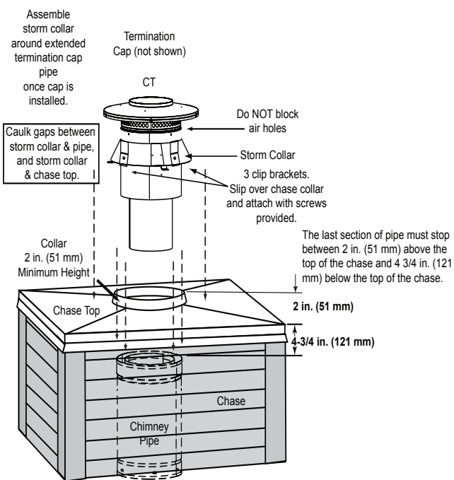
Figure 5.15 Installing a DTO134/DTO146/DTS134/DTS146 Cap
