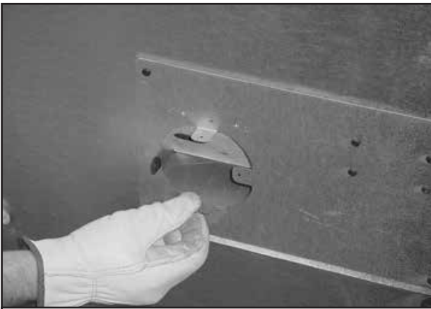
Figure 3.18 Bending Tabs on Outside Air Kit Collar
