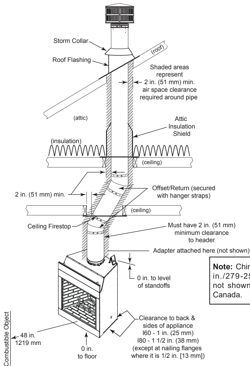
Figure 3.3 Clearances to Combustible Materials
