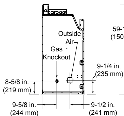
Figure 3.1 Appliance Dimensions
