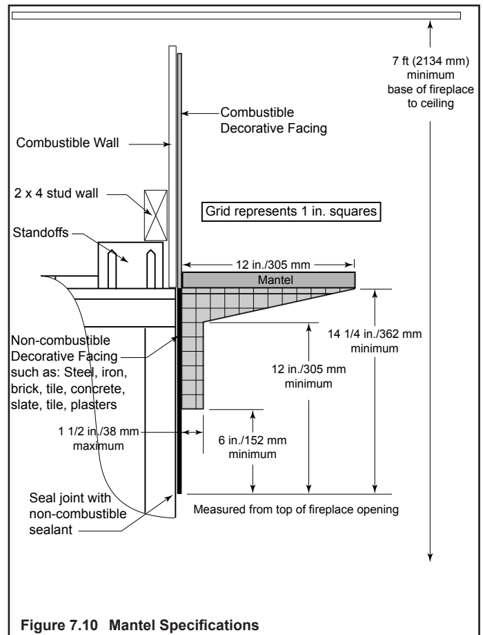
Figure 7.10 Mantel Specifications
