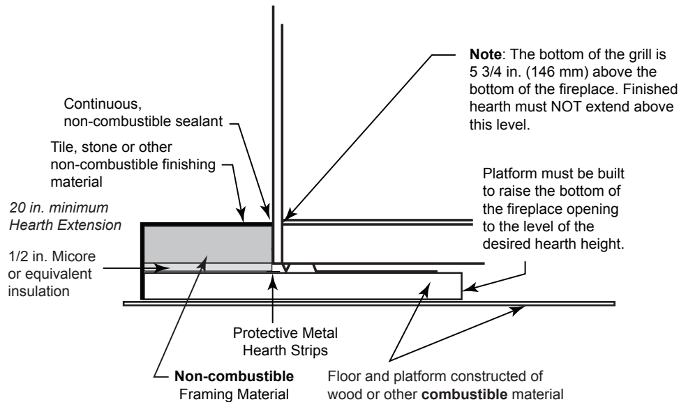
Figure 7.8 Raised Hearth Extension and Fireplace Framing Materials
