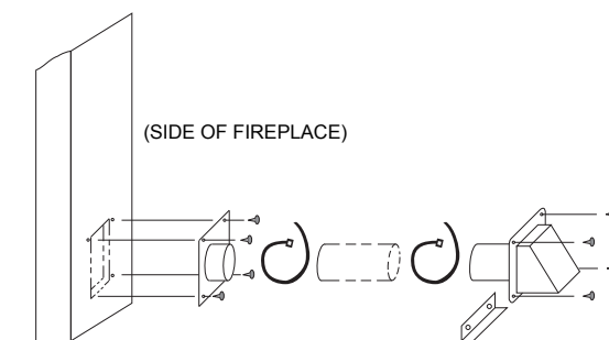
AK14/AK18 Outside Air Kit
