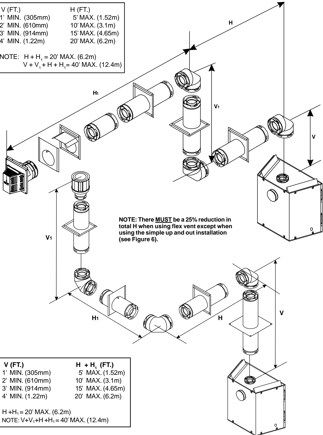
Figure 17. Venting with three 90° elbows
