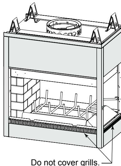
Figure 11.2 Non-combustible Materials Zone
