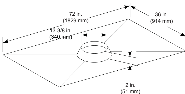
TCT1175 - Terra Cotta Cap
