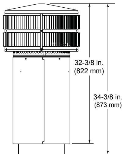
TR11T - Round Telescoping Termination Cap
