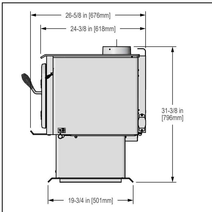
Figure 8.3 - Side View
