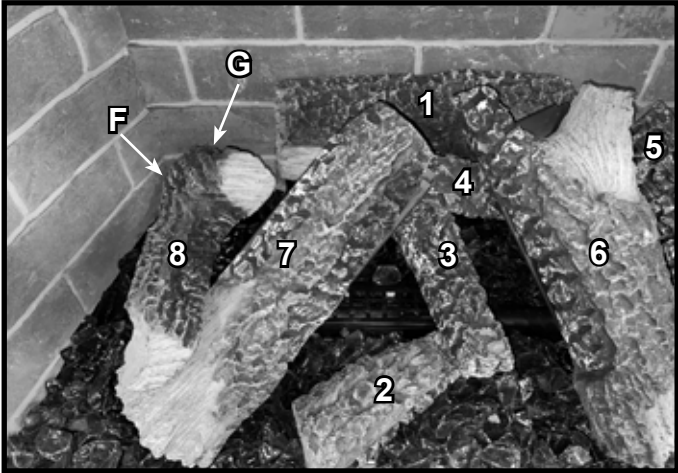
Figure 17 Log #8 Installed
