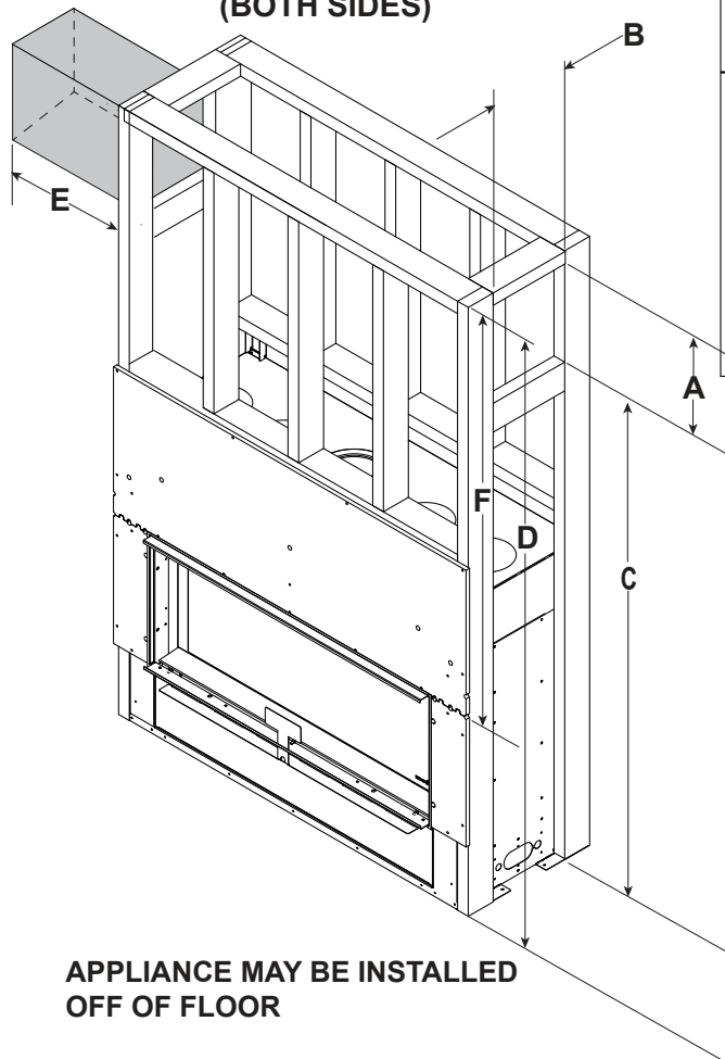
SIDE DISCHARGE FRAMING DIMENSIONS
