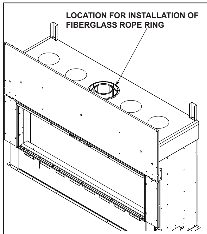
Figure 6.3 Location of Fiberglass Rope Ring
