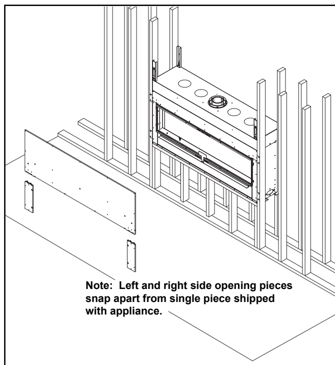
Figure 6.9 Install Factory-Included Non-Combustible Facing Material
