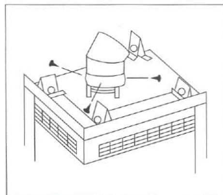
Figure 13 Offset Secured to Fireplace
