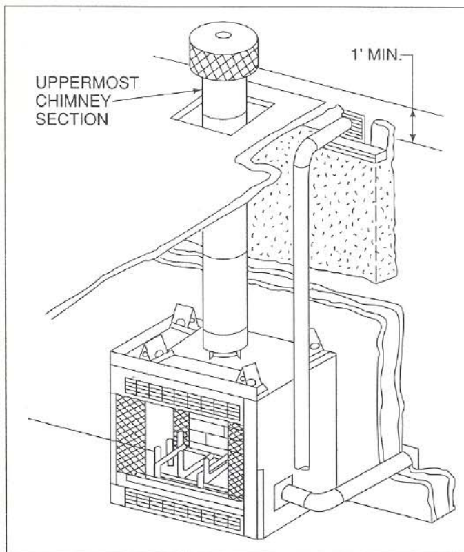
Figure 12 Outside Air Locations
