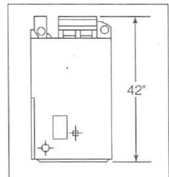
Figure 9 Fireplace (Side View)
