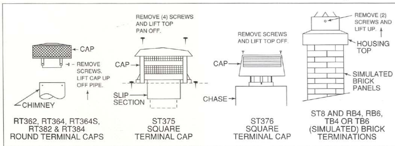
Figure 20 Terminal Caps
