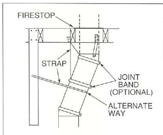
Figure 16 Offset/Return Installation
