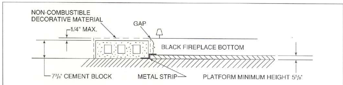
Figure 6 Field Constructed Hearth Extension
