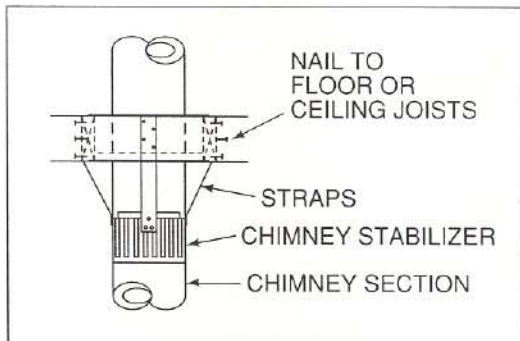
Figure 15 Chimney with Stabilizer
