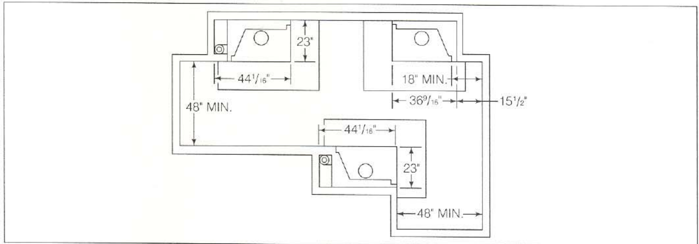
Figure 1 Fireplace Locations
