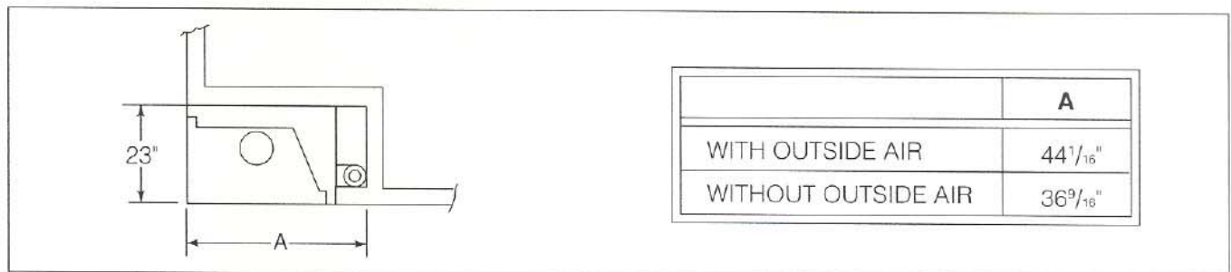
Figure 2 Minimum Clearances to Combustibles With Outside Air
