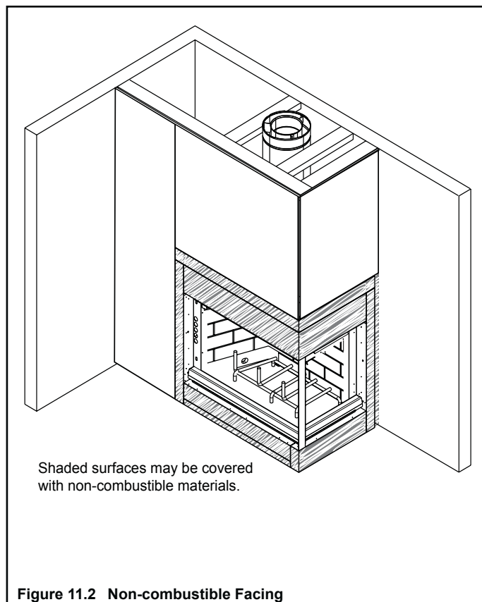
Figure 11.2 Non-combustible Facing
