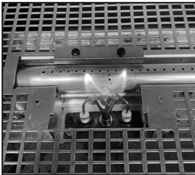
Figure 4.18 IPI Pilot Flame Patterns
