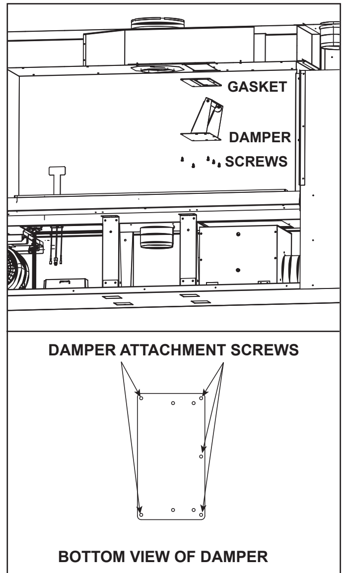
Figure 4.20 Damper Replacement
