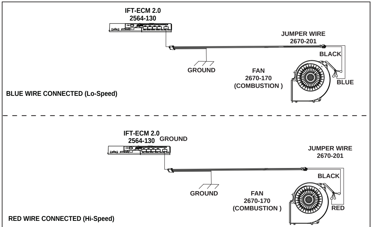
Figure 4.12 Fan Speed Wiring Diagram
