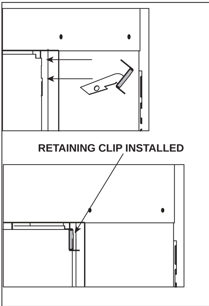
Figure 11.26 Barrier Glass Retaining Clip Installation (Right Side Shown)
