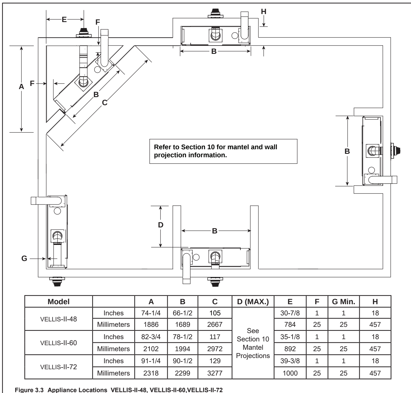
Figure 3.3 Appliance Locations VELLIS-II-48, VELLIS-II-60, VELLIS-II-72
