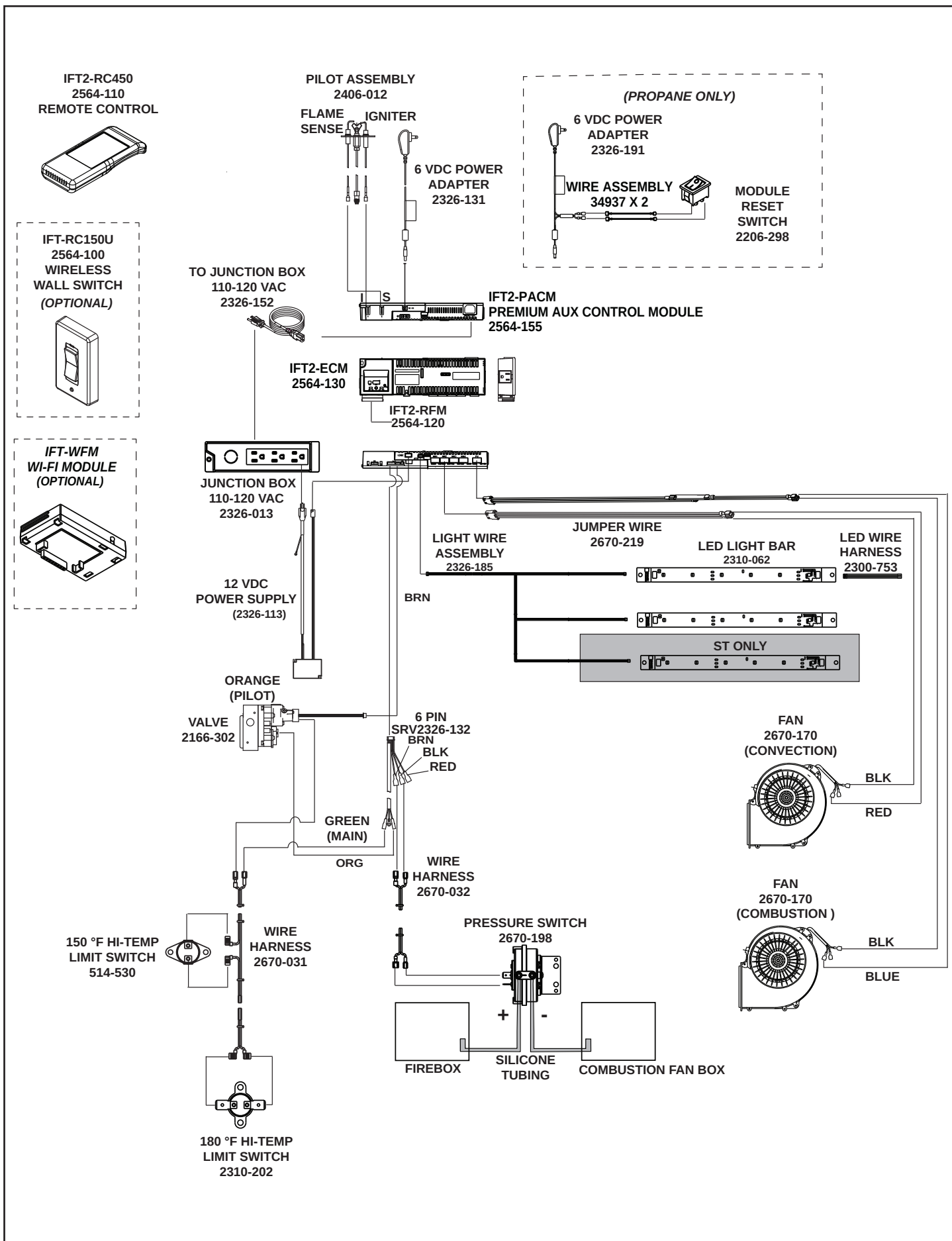
➔ Figure 8.7 IntelliFire Touch Wiring Diagram
