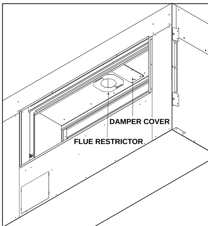
Figure 4.13 Flue Restrictor Location in Appliance
