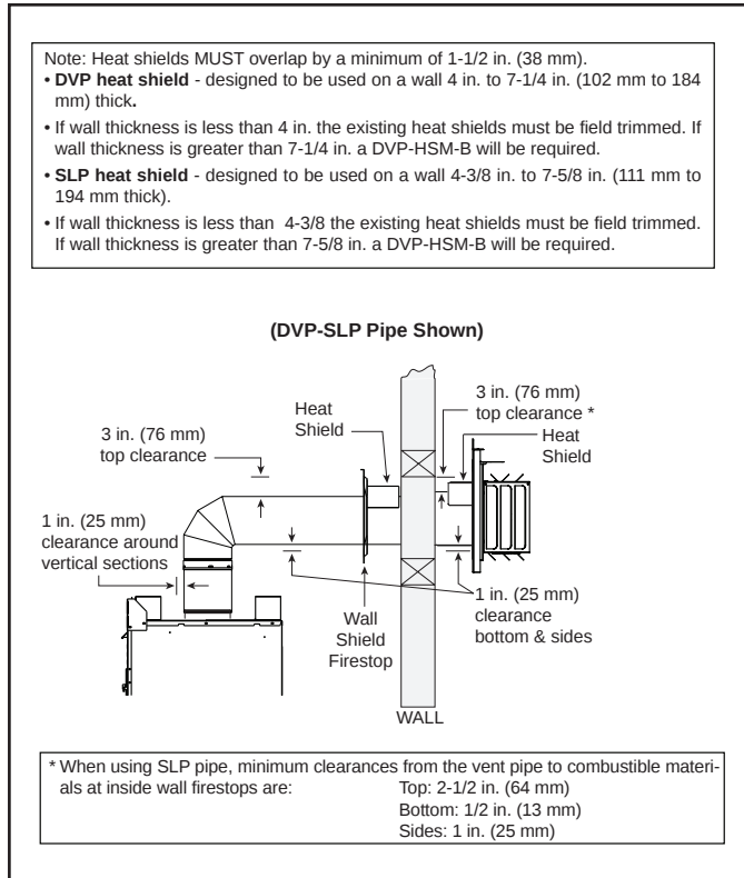
Figure 5.1 Horizontal Venting Clearances To Combustible Materials
