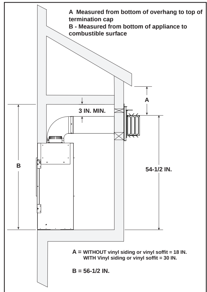
Figure 3.9 Exterior Chase - Minimum Height Requirements
