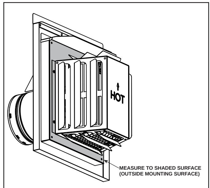
Figure 4.9 Measure to Outside Mounting Surface
