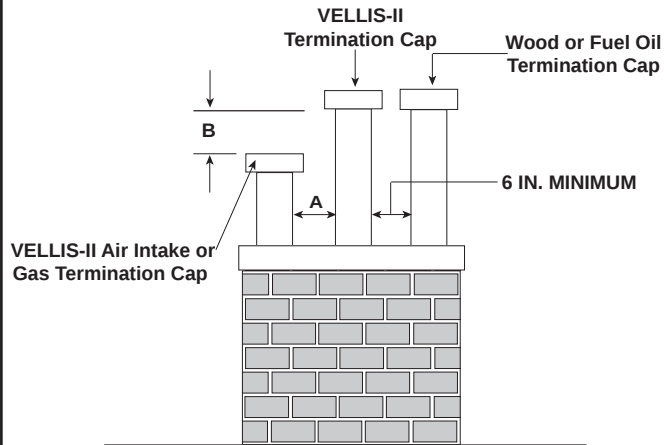
Figure 4.2 Staggered Termination Caps
