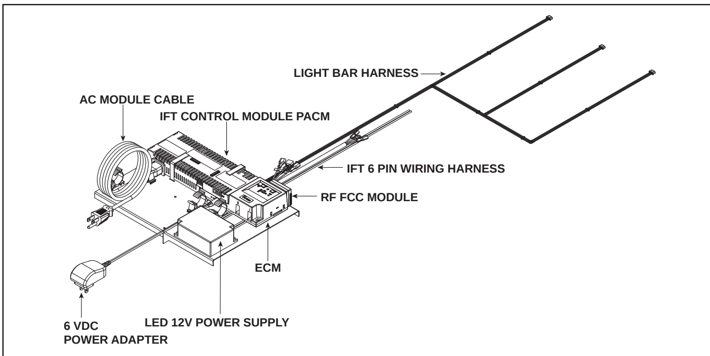
Figure 8.6 Component Tray Assembled
