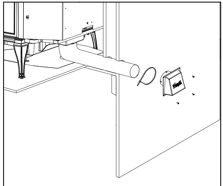
Figure 5.12 - Installation arrière
