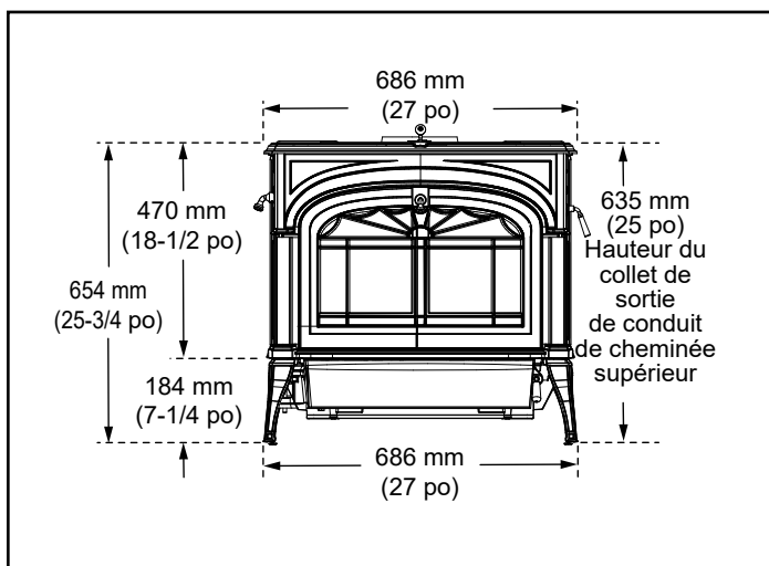
Figure 3.1 – Vue frontale
