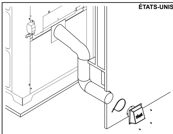
Figure 16.2 - Installation au sol
