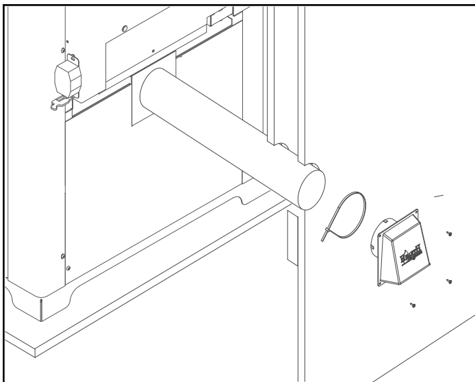
Figure 16.1 - Installation arrière
