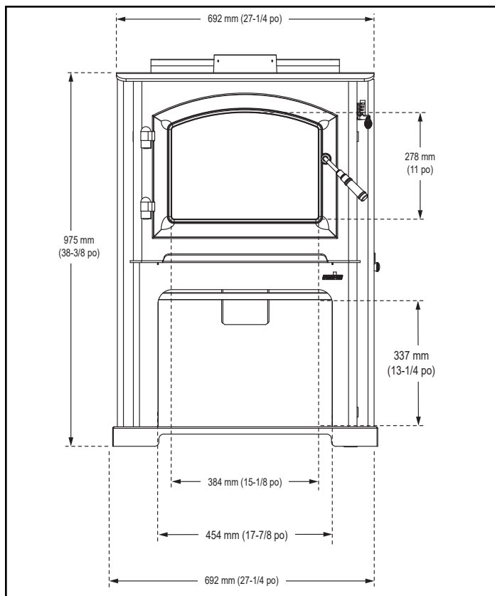
Figure 8.1 - Vue frontale
