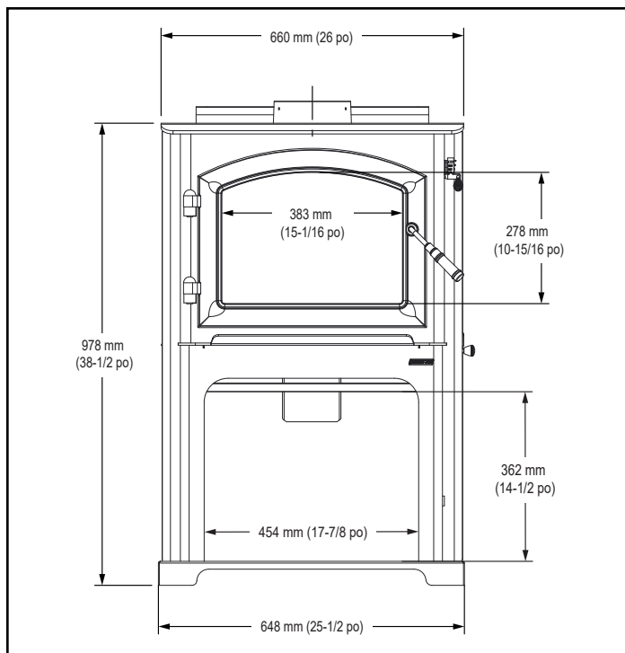
Figure 8.1 - Vue frontale
