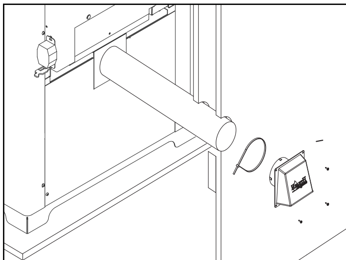
Figure 16.1 - Installation arrière
