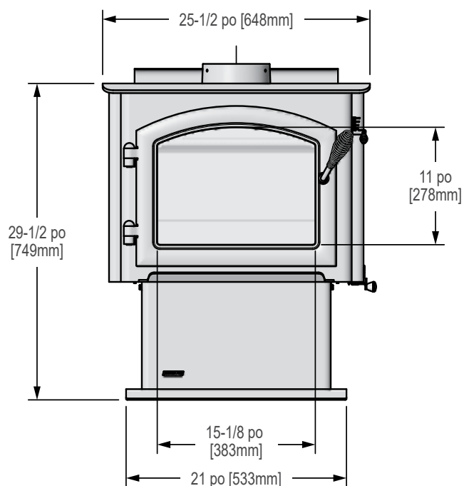
Figure 8.1 – Vue frontale
