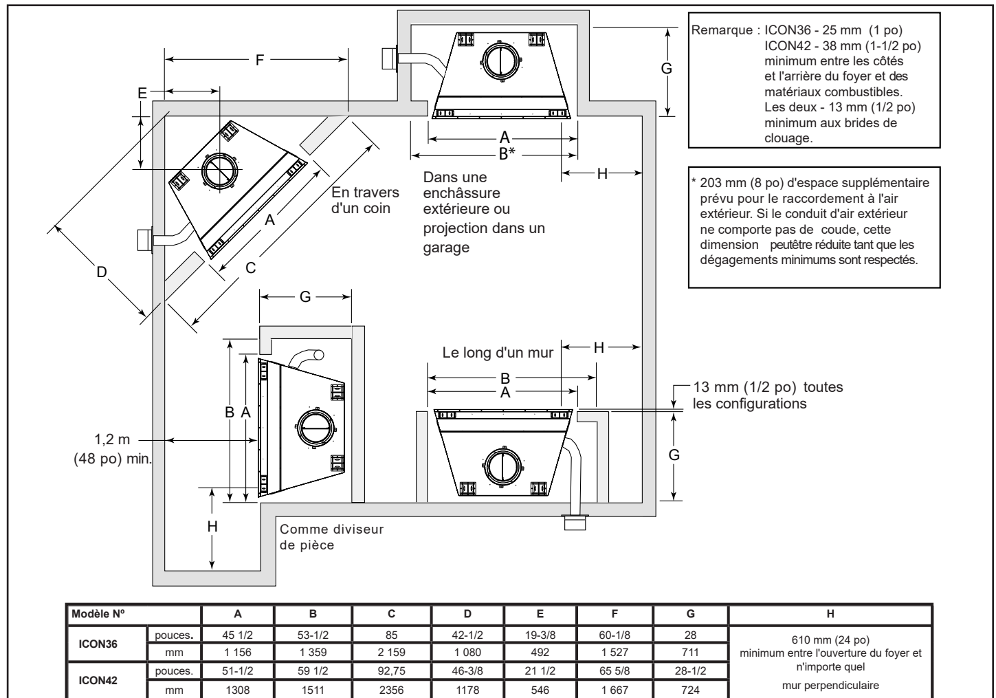
Figure 2.2 Emplacements des foyers
