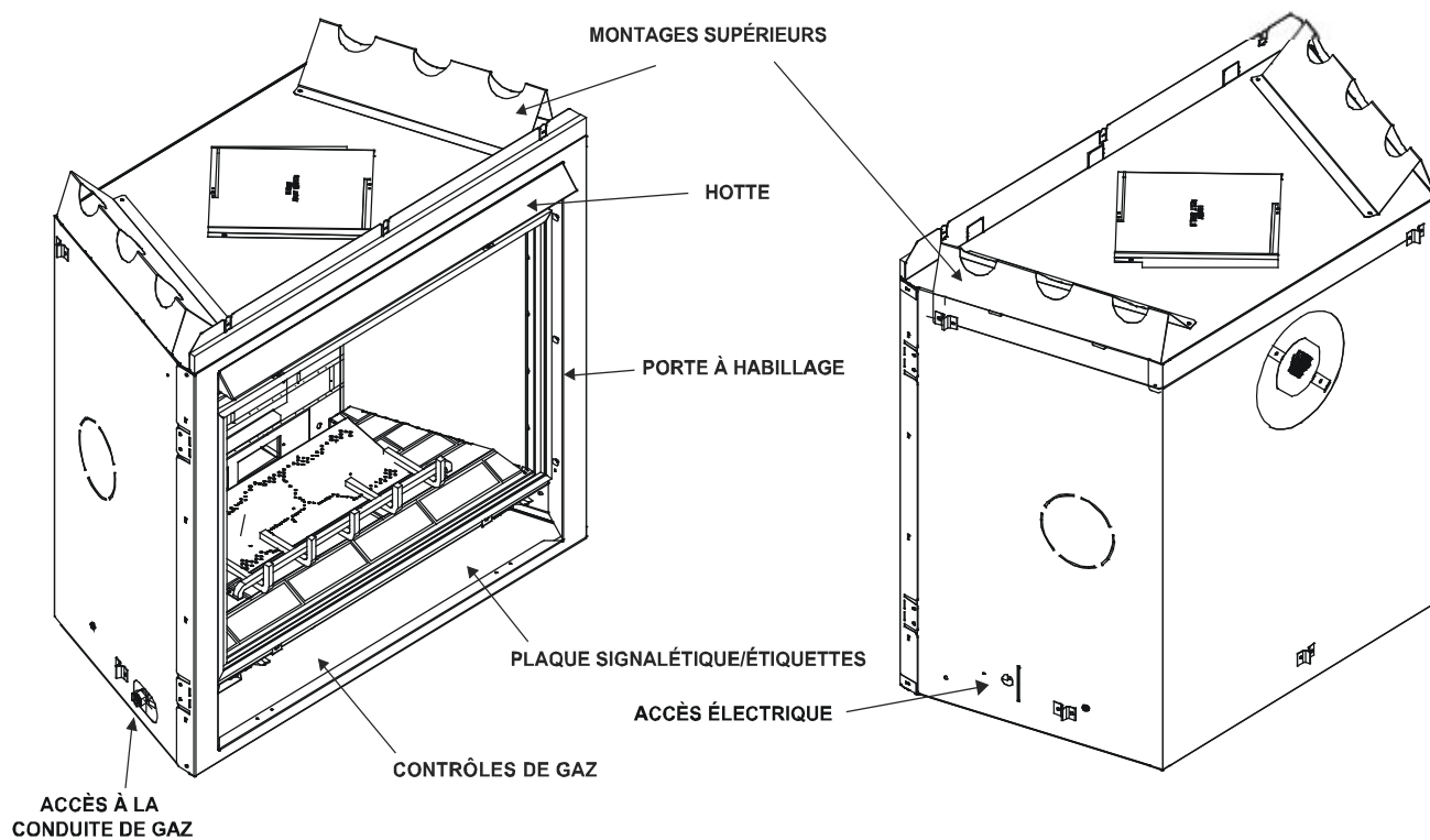
Figure 1. Diagramme de QV36D
