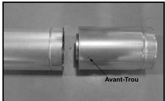
Figure 8.7 Avant-trous de la section coulissante
