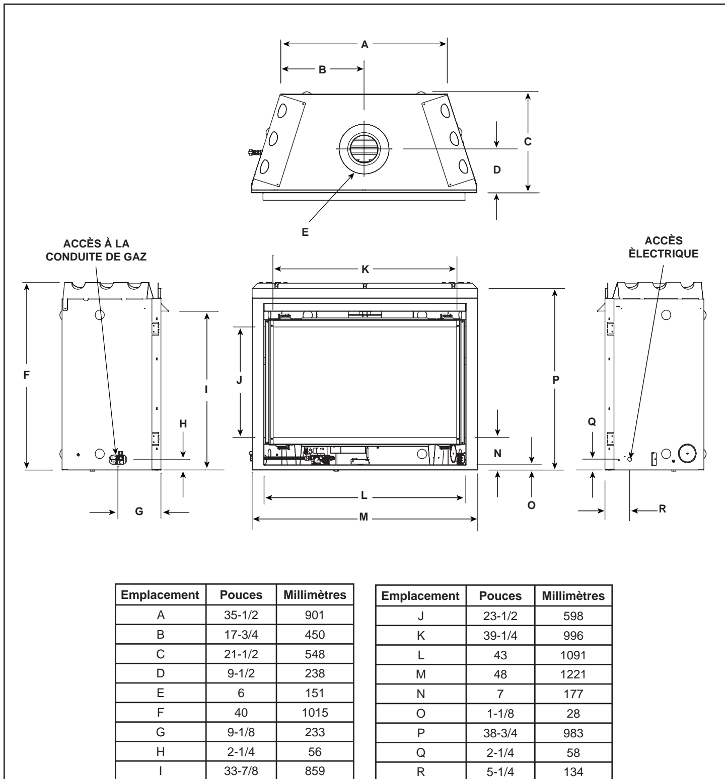
Figure 16.1 Dimensions du foyer
