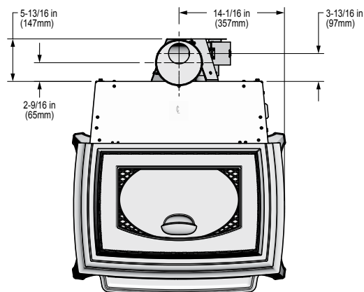
Figure 8.4 - Top View with Top Vent Adapter (TPVNT-3) and Offset Adapter (812-3570).
