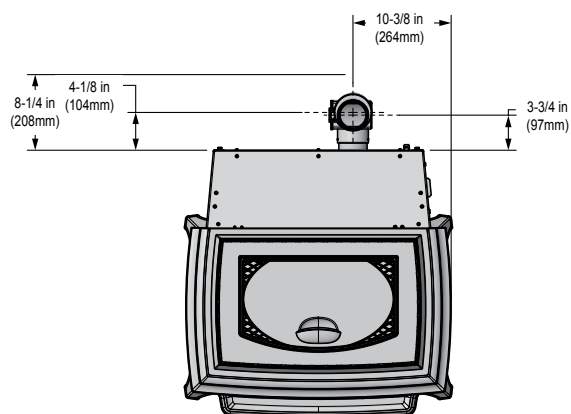
Figure 8.5 - Top View with Top Vent Adapter (TPVNT-6) and Offset Adapter (811-0720).
