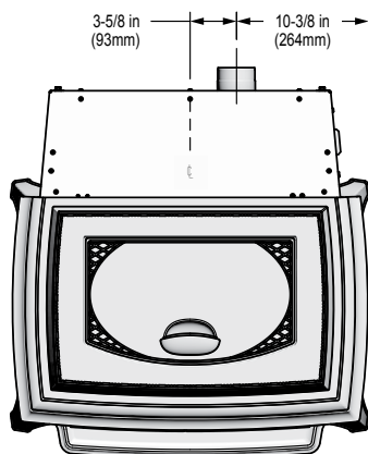
Figure 8.1 - Top View
