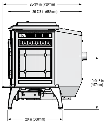
Figure 9.1 -Side View
