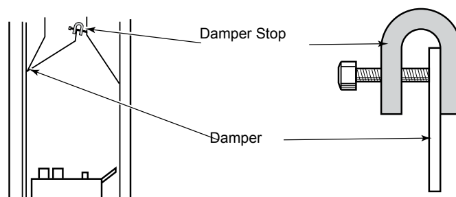
Figure 3.8 - Damper Stop Installation.
