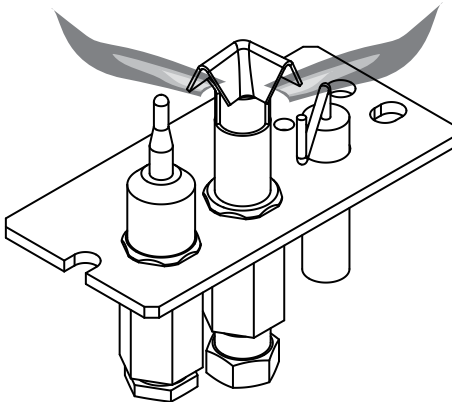
Figure 6.15 - Incorrect Appearance of Pilot Flame
